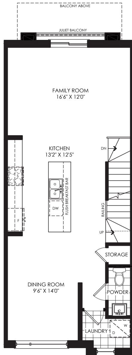
MAIN FLOOR ELEV. 'A'
