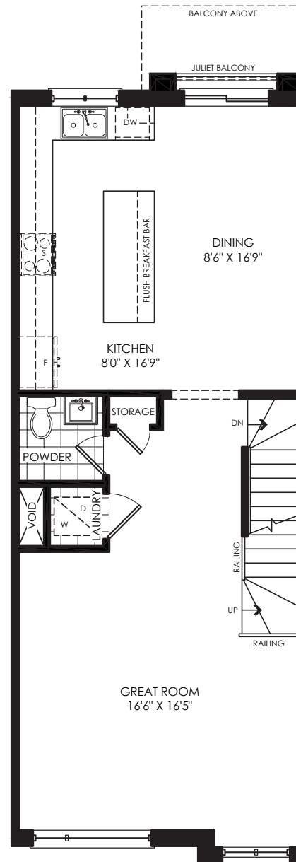
MAIN FLOOR ELEV. 'A'
